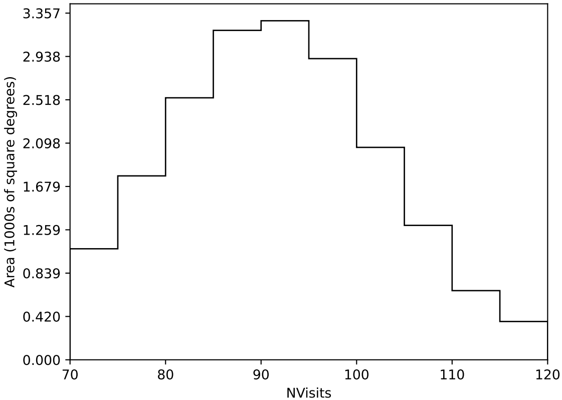
too_elab_r64_d2_gz_v3.4_10yrs Yr 1 all bands: NVisits
