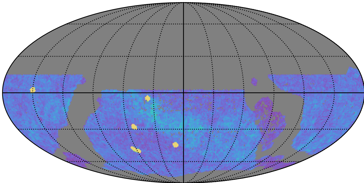
too_elab_r64_d2_gz_v3.4_10yrs WFD z band: NVisits
