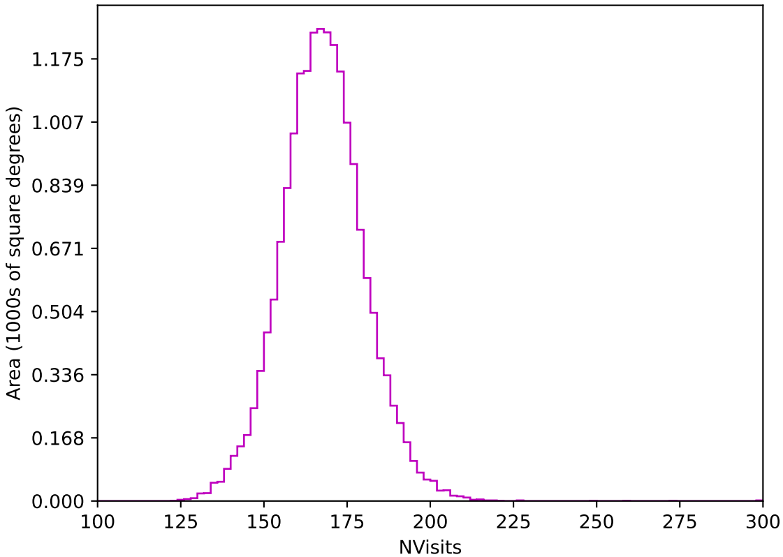
too_elab_r64_d2_gz_v3.4_10yrs WFD z band: NVisits
