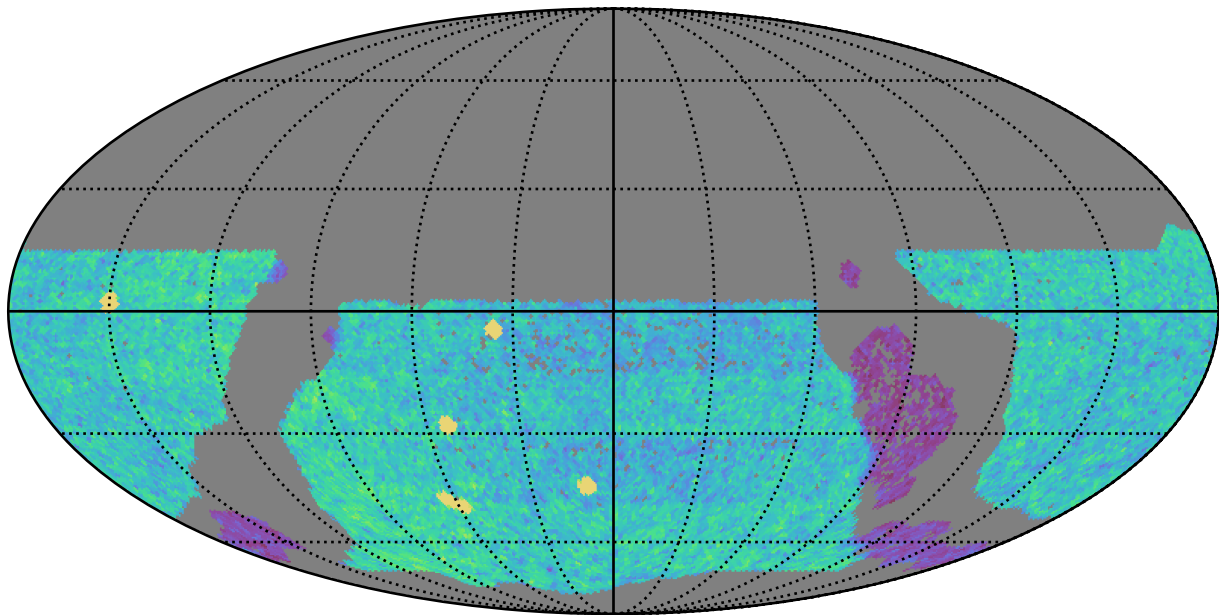
too_elab_r64_d2_gz_v3.4_10yrs WFD u band: NVisits
