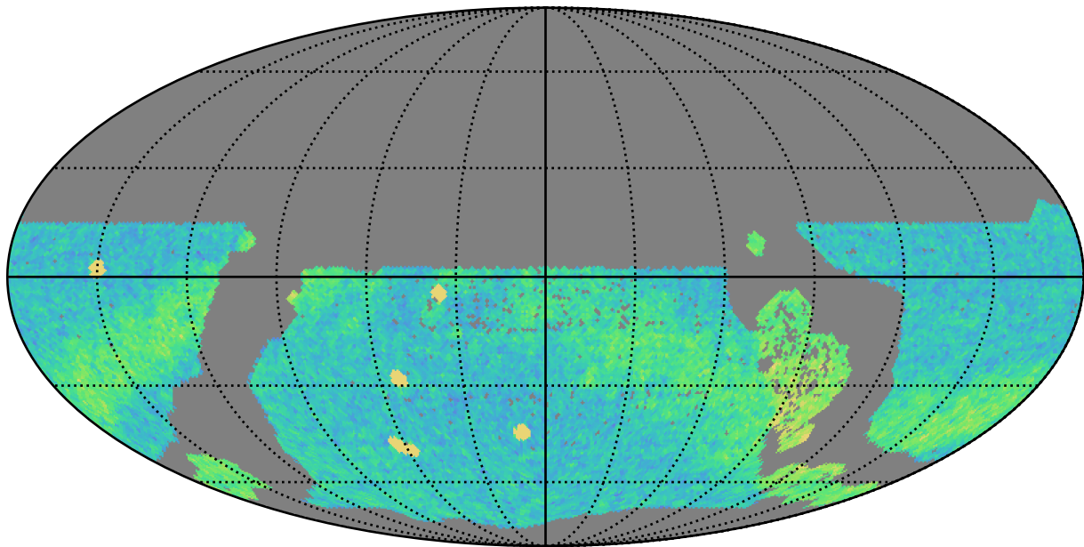
too_elab_r64_d2_gz_v3.4_10yrs WFD r band: NVisits
