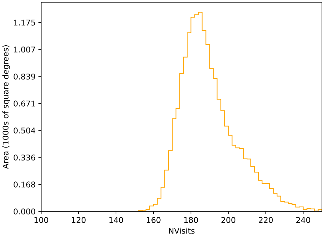
too_elab_r64_d2_gz_v3.4_10yrs WFD r band: NVisits
