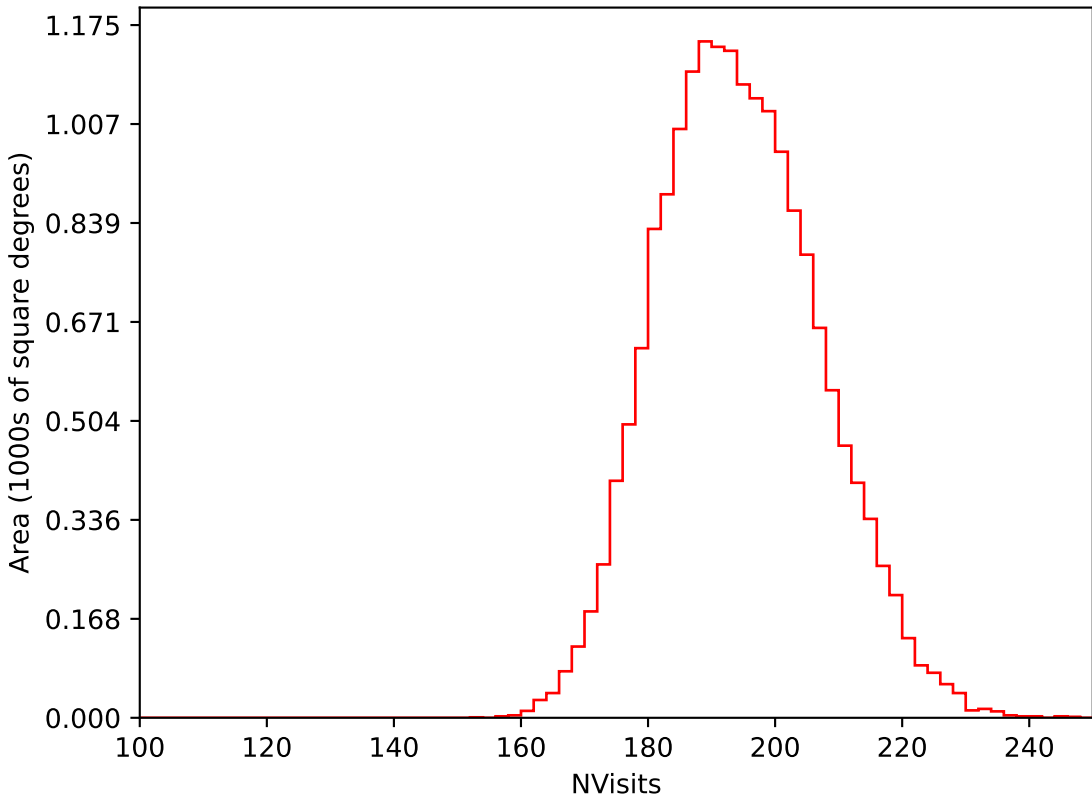
too_elab_r64_d2_gz_v3.4_10yrs WFD i band: NVisits
