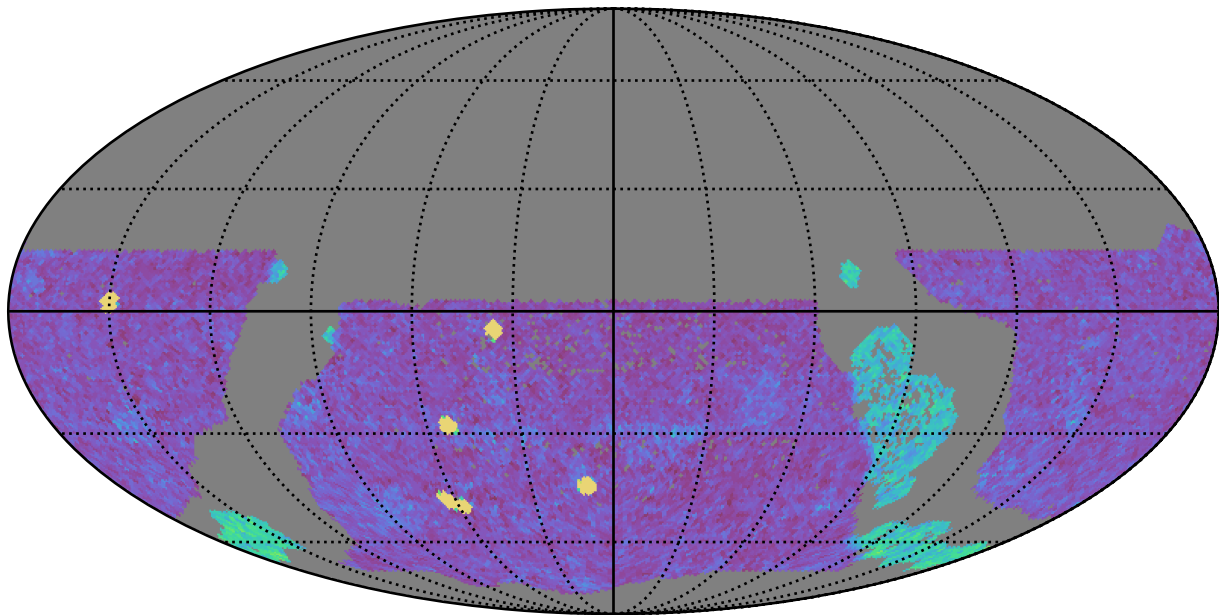
too_elab_r64_d2_gz_v3.4_10yrs WFD g band: NVisits
