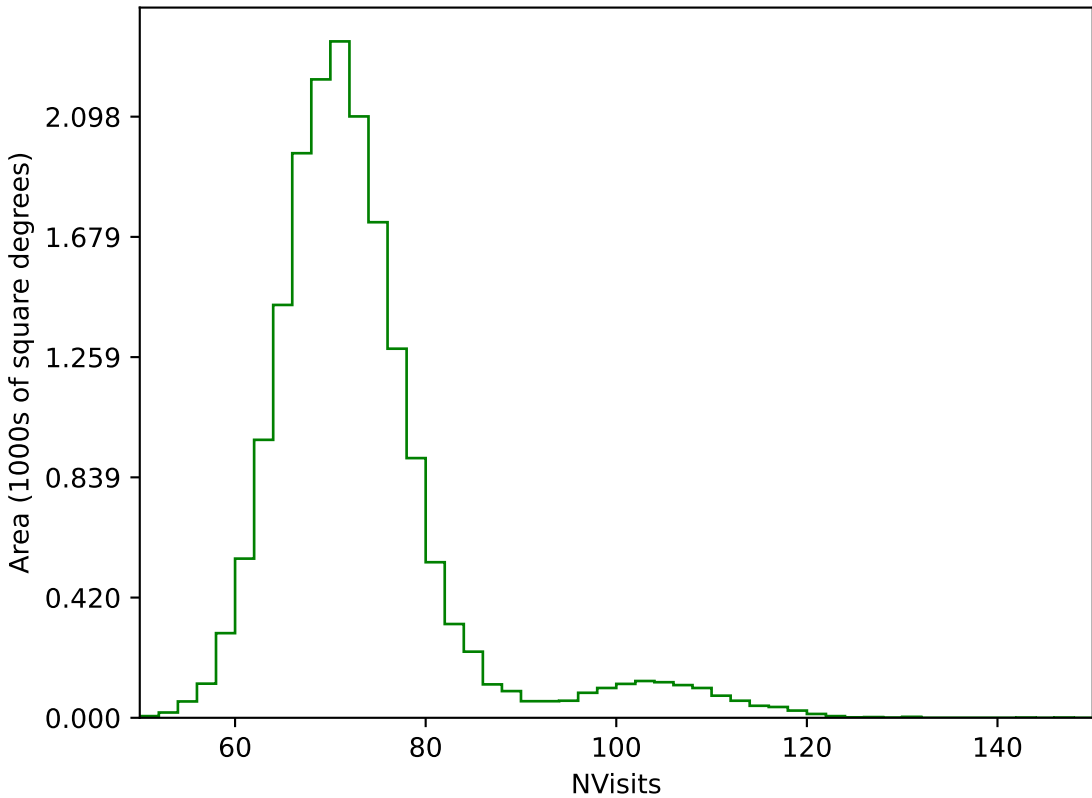
too_elab_r64_d2_gz_v3.4_10yrs WFD g band: NVisits
