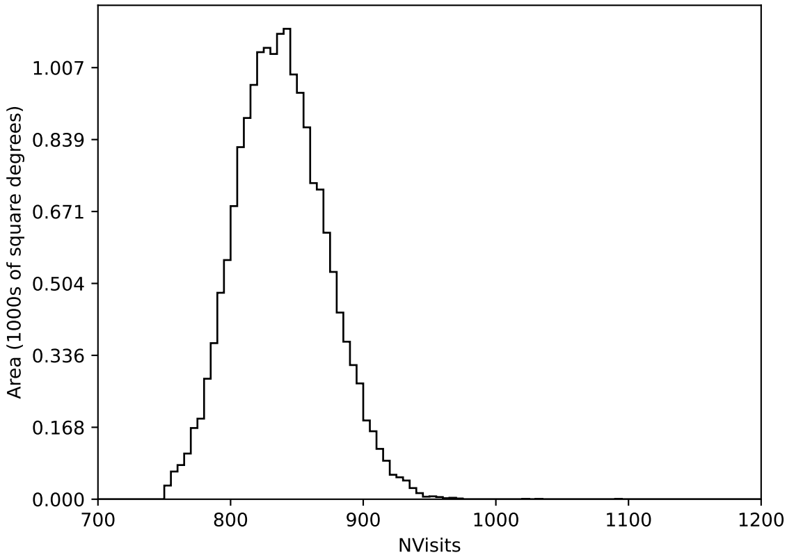
too_elab_r64_d2_gz_v3.4_10yrs WFD all bands: NVisits
