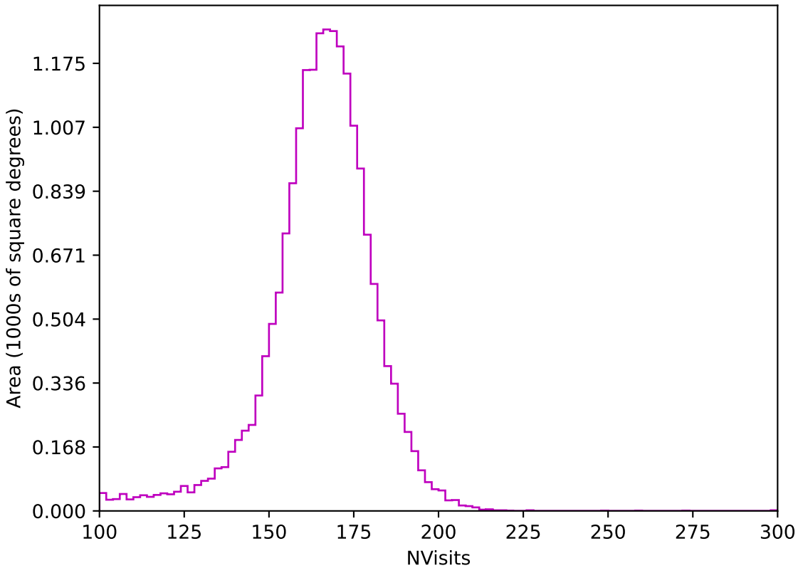
too_elab_r64_d2_gz_v3.4_10yrs All sky z band: NVisits
