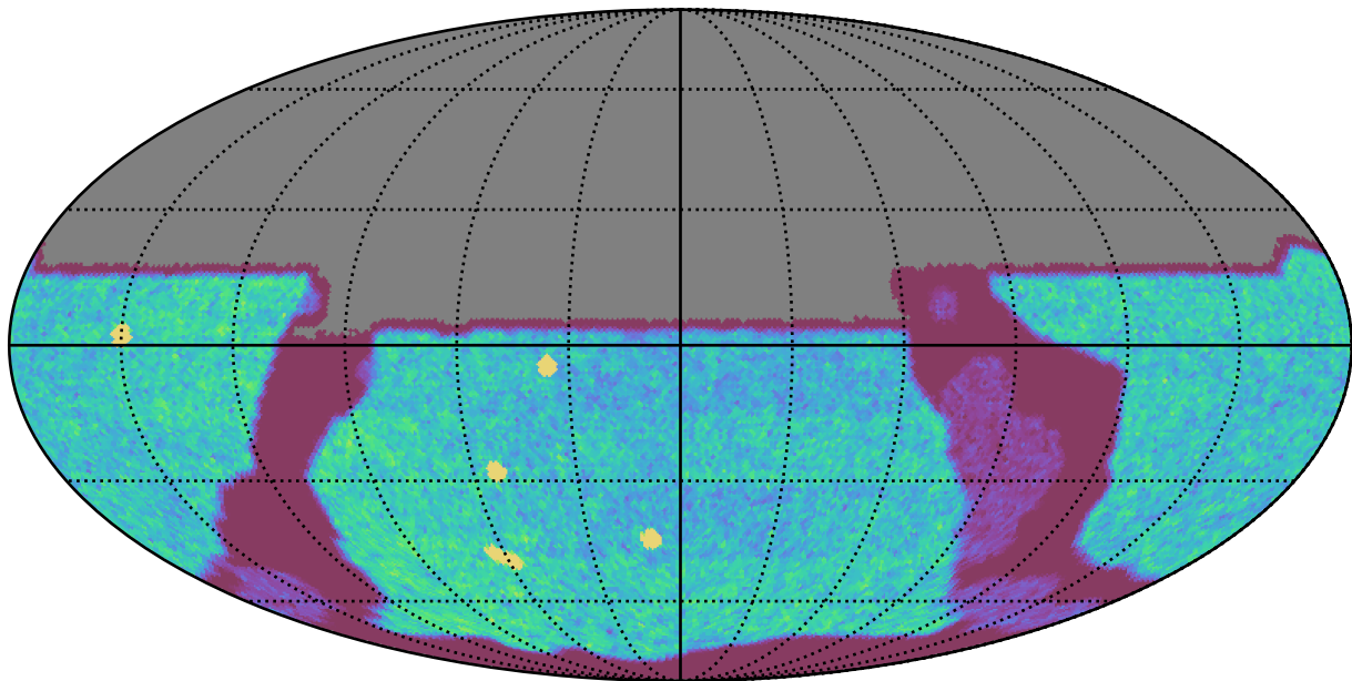
too_elab_r64_d2_gz_v3.4_10yrs All sky u band: NVisits
