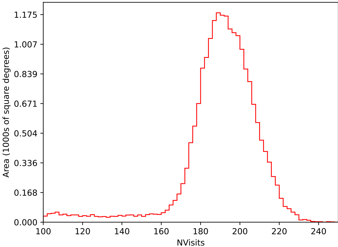
too_elab_r64_d2_gz_v3.4_10yrs All sky i band: NVisits
