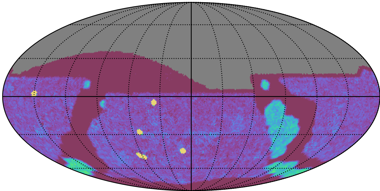
too_elab_r64_d2_gz_v3.4_10yrs All sky g band: NVisits
