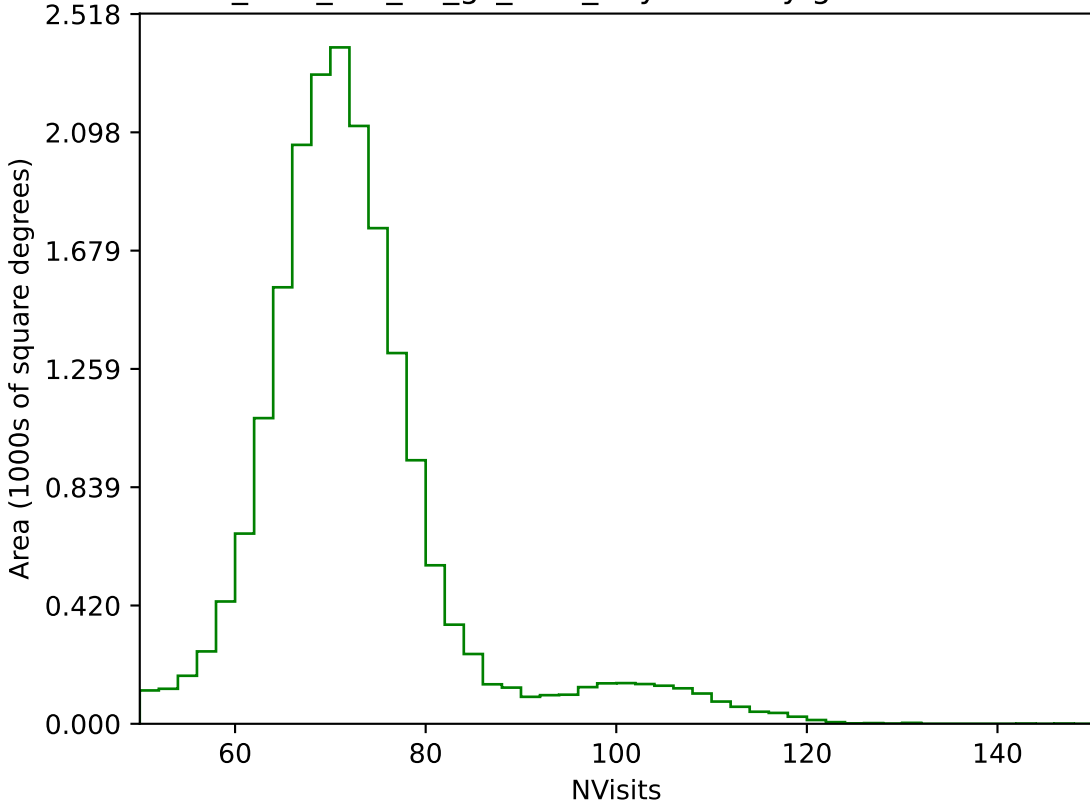
too_elab_r64_d2_gz_v3.4_10yrs All sky g band: NVisits
