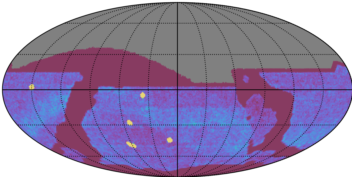
too_elab_r64_d2_gz_v3.4_10yrs All sky all bands: NVisits
