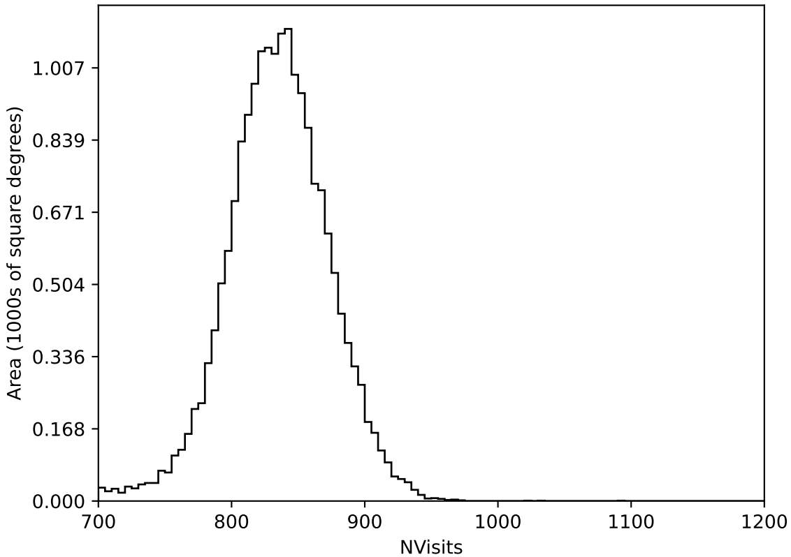
too_elab_r64_d2_gz_v3.4_10yrs All sky all bands: NVisits
