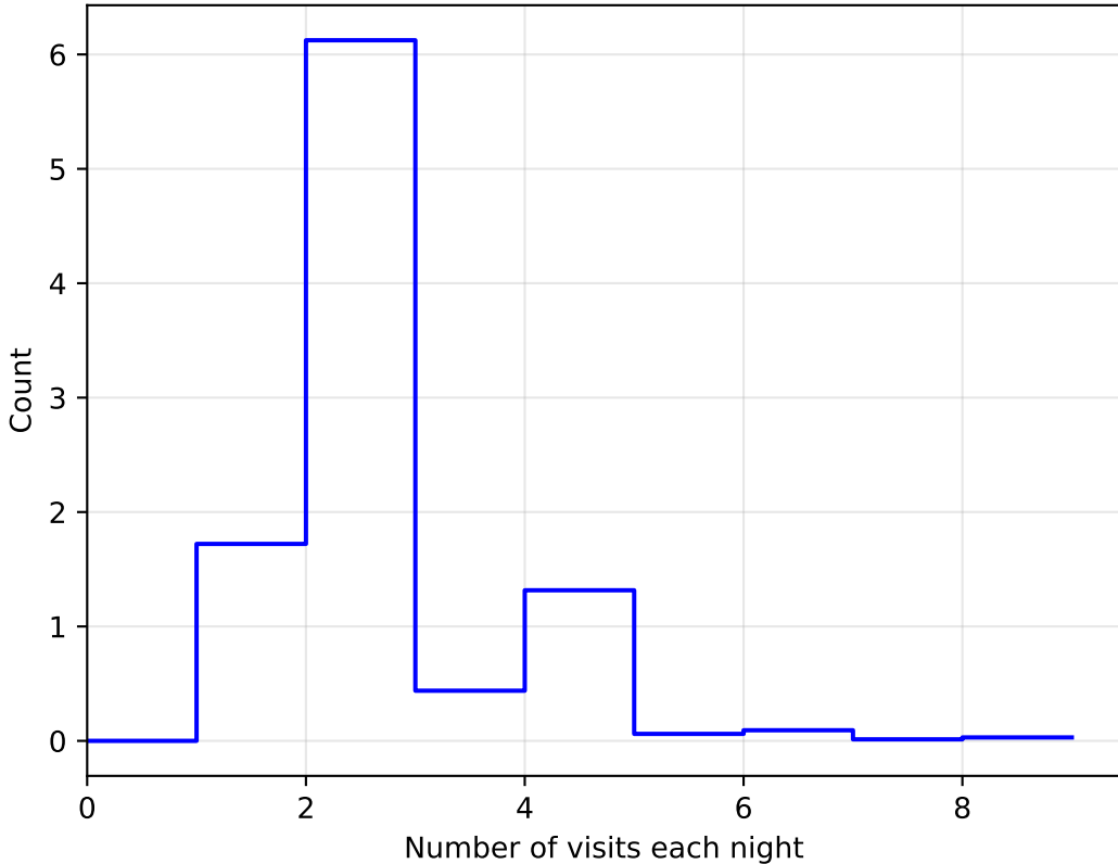
too_elab_r64_d2_gz_v3.4_10yrs All sky: NVisitsPerNight
