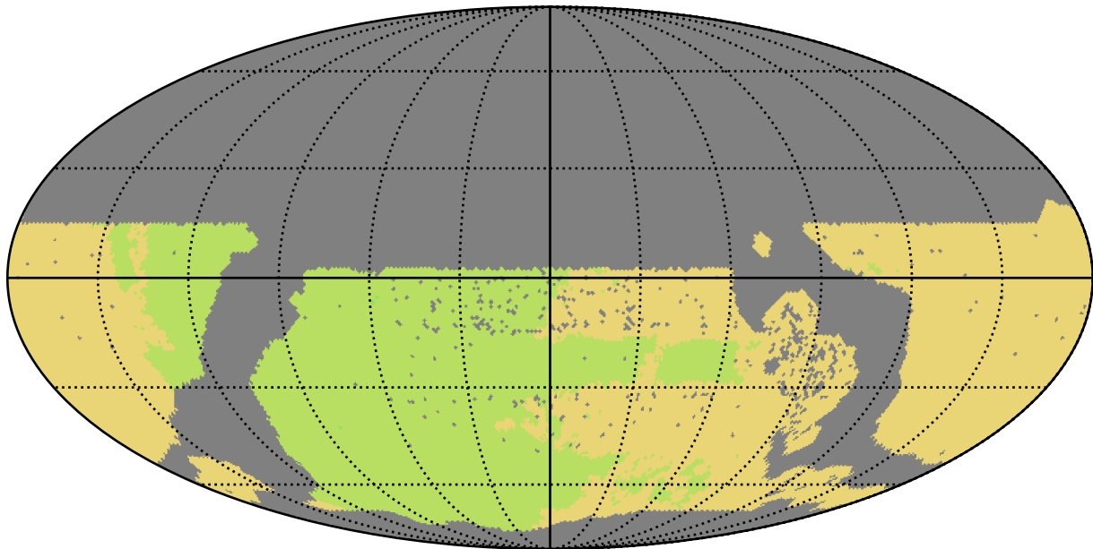
too_elab_r64_d2_gz_v3.4_10yrs WFD all bands: NSeasons
