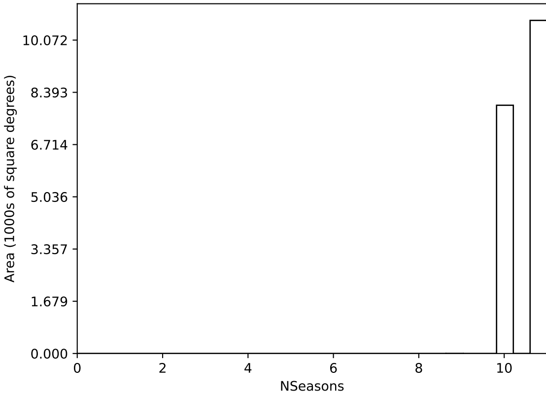
too_elab_r64_d2_gz_v3.4_10yrs WFD all bands: NSeasons
