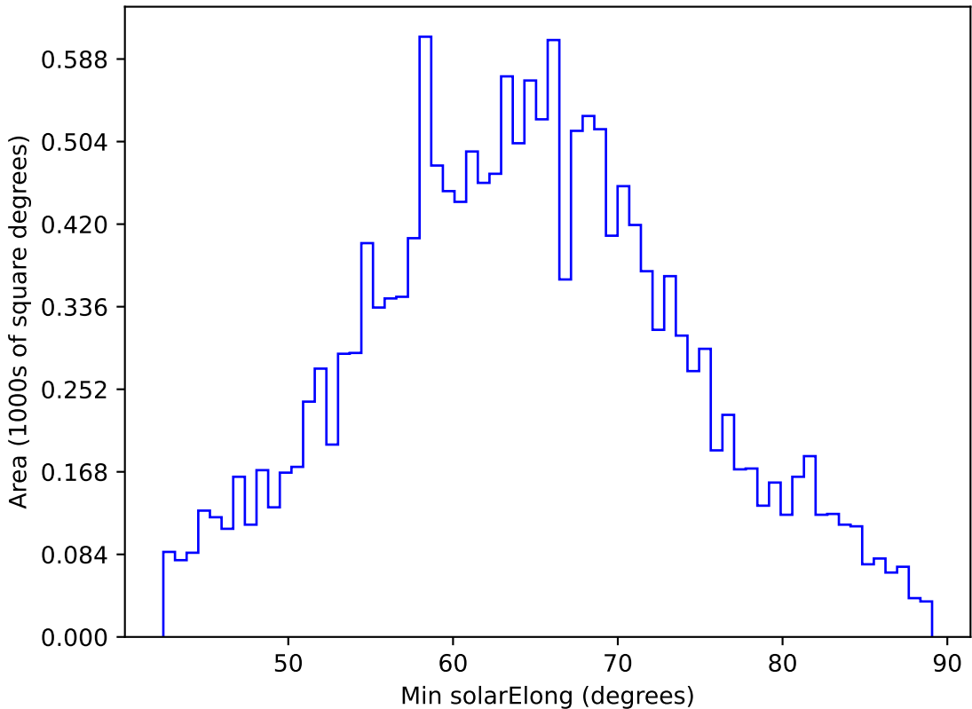
too_elab_r64_d2_gz_v3.4_10yrs WFD y band: Min solarElong
