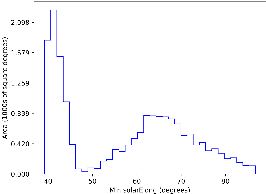
too_elab_r64_d2_gz_v3.4_10yrs WFD r band: Min solarElong
