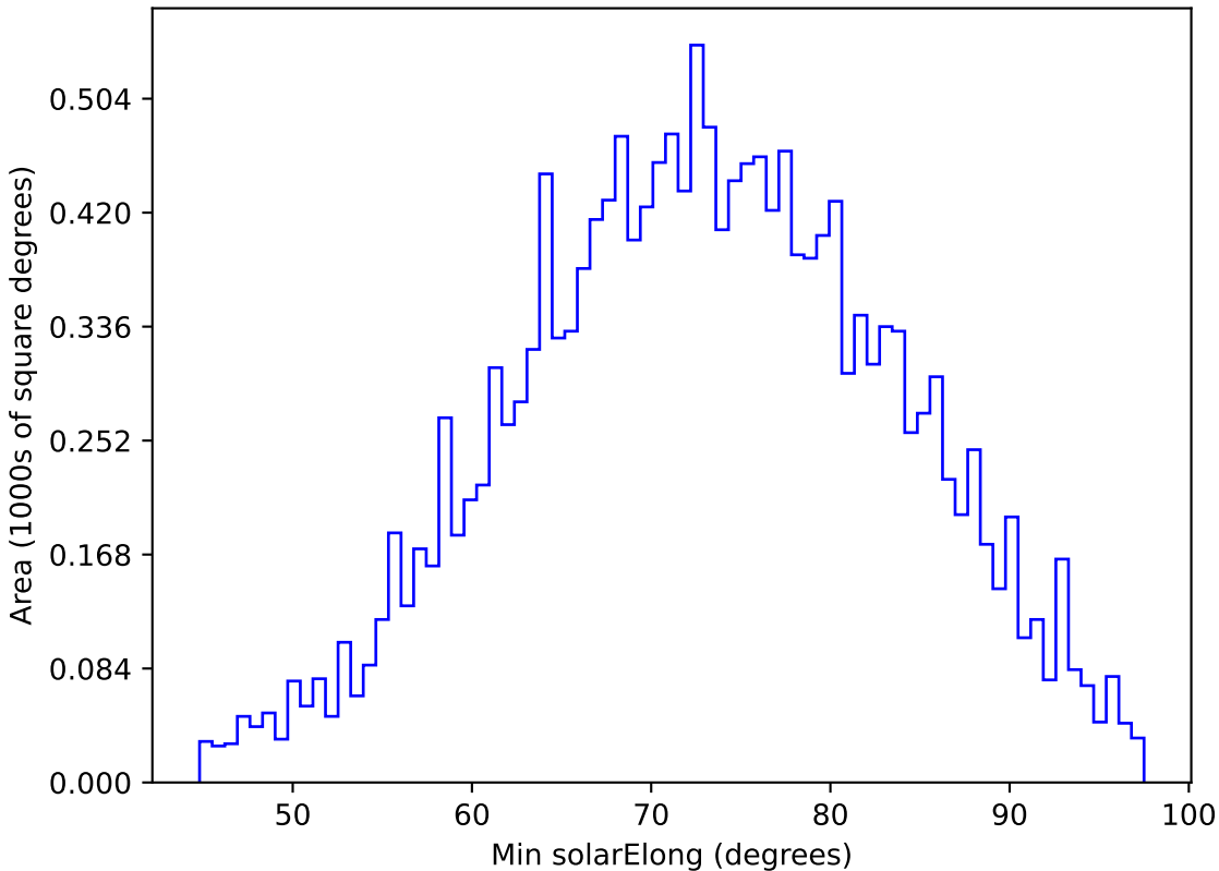
too_elab_r64_d2_gz_v3.4_10yrs WFD g band: Min solarElong
