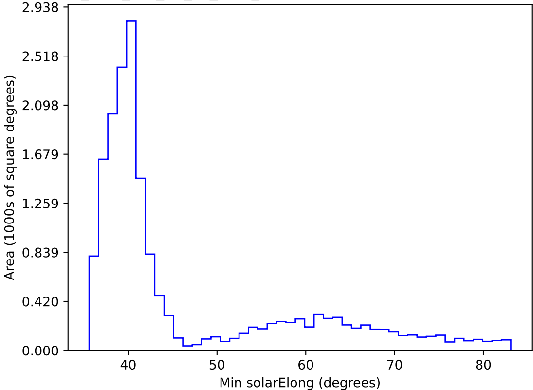
too_elab_r64_d2_gz_v3.4_10yrs WFD all bands: Min solarElong
