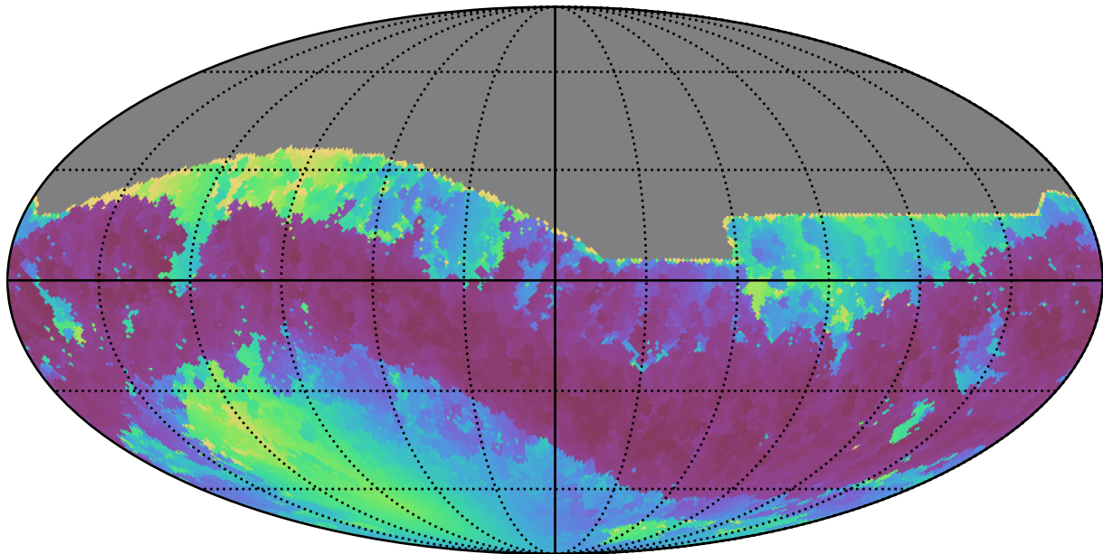
too_elab_r64_d2_gz_v3.4_10yrs All sky z band: Min solarElong
