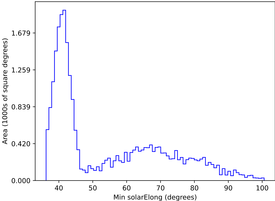
too_elab_r64_d2_gz_v3.4_10yrs All sky z band: Min solarElong
