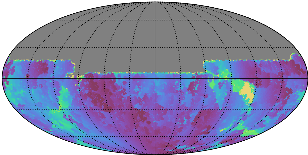
too_elab_r64_d2_gz_v3.4_10yrs All sky u band: Min solarElong
