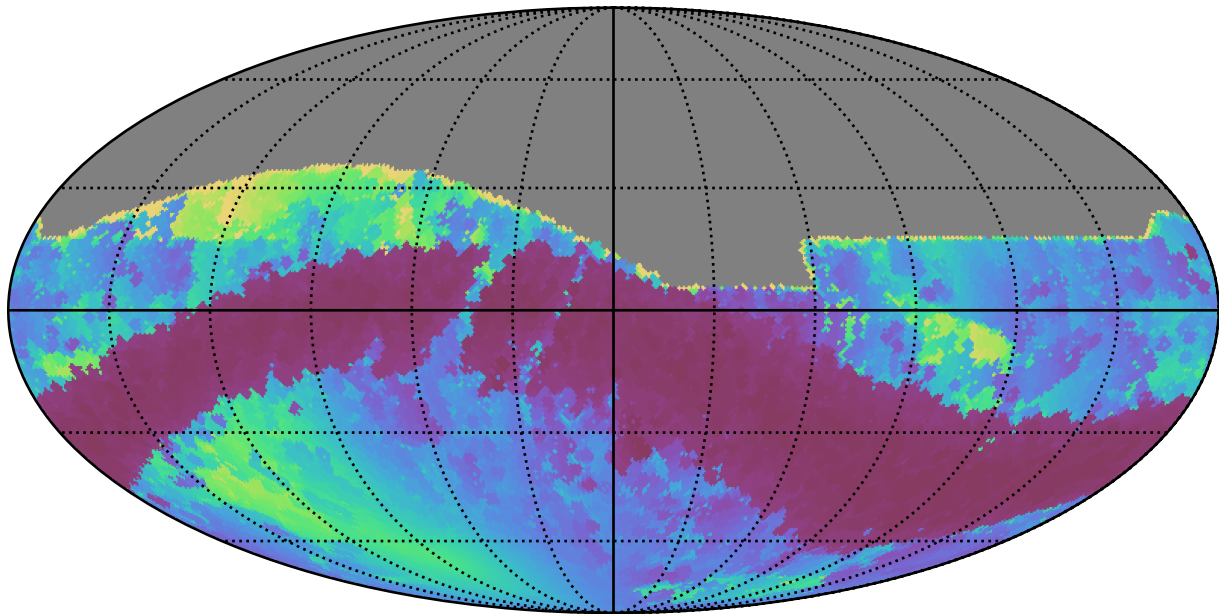
too_elab_r64_d2_gz_v3.4_10yrs All sky r band: Min solarElong
