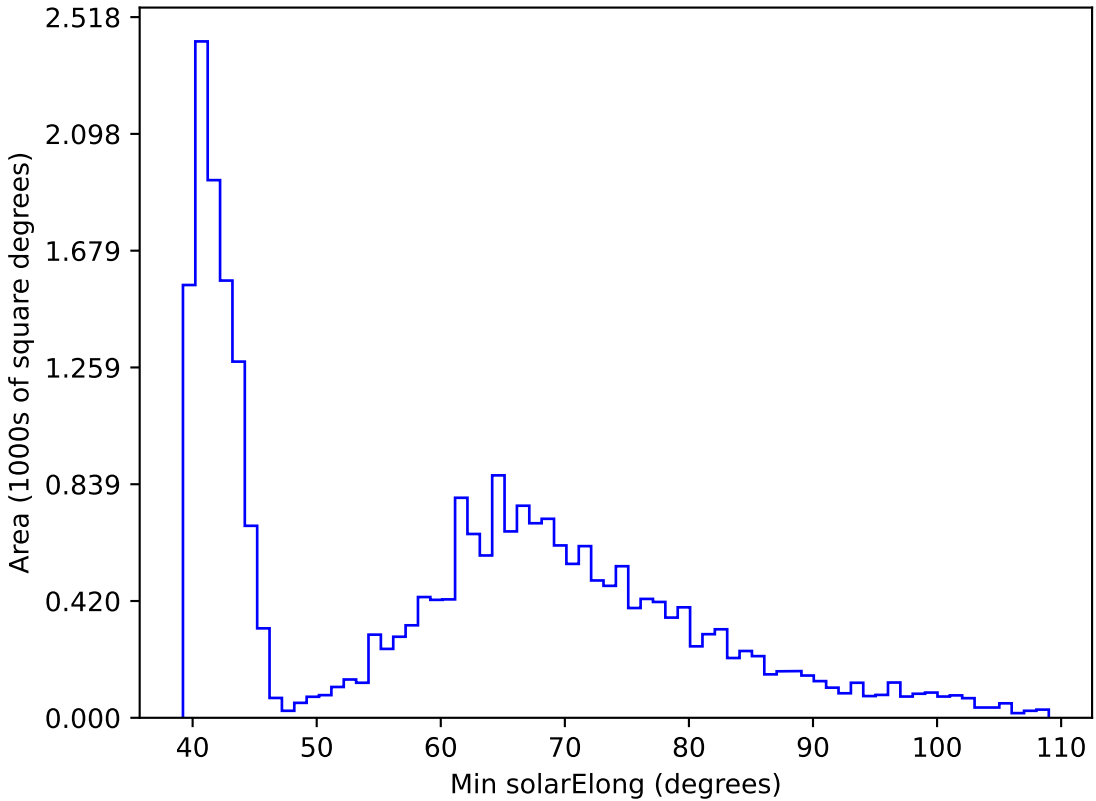
too_elab_r64_d2_gz_v3.4_10yrs All sky r band: Min solarElong
