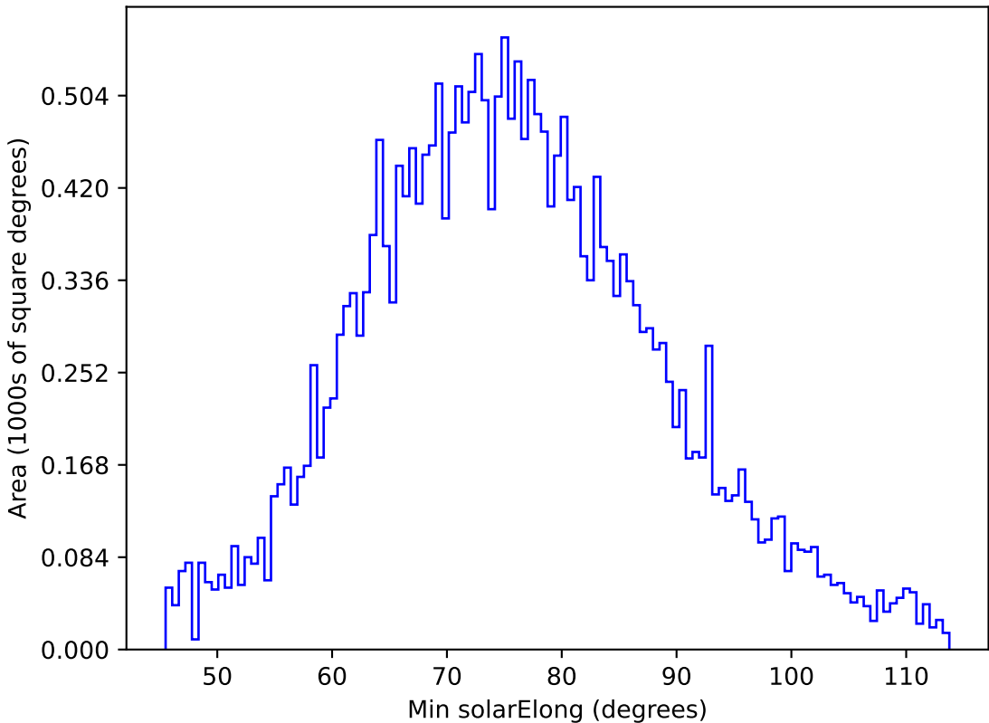
too_elab_r64_d2_gz_v3.4_10yrs All sky g band: Min solarElong
