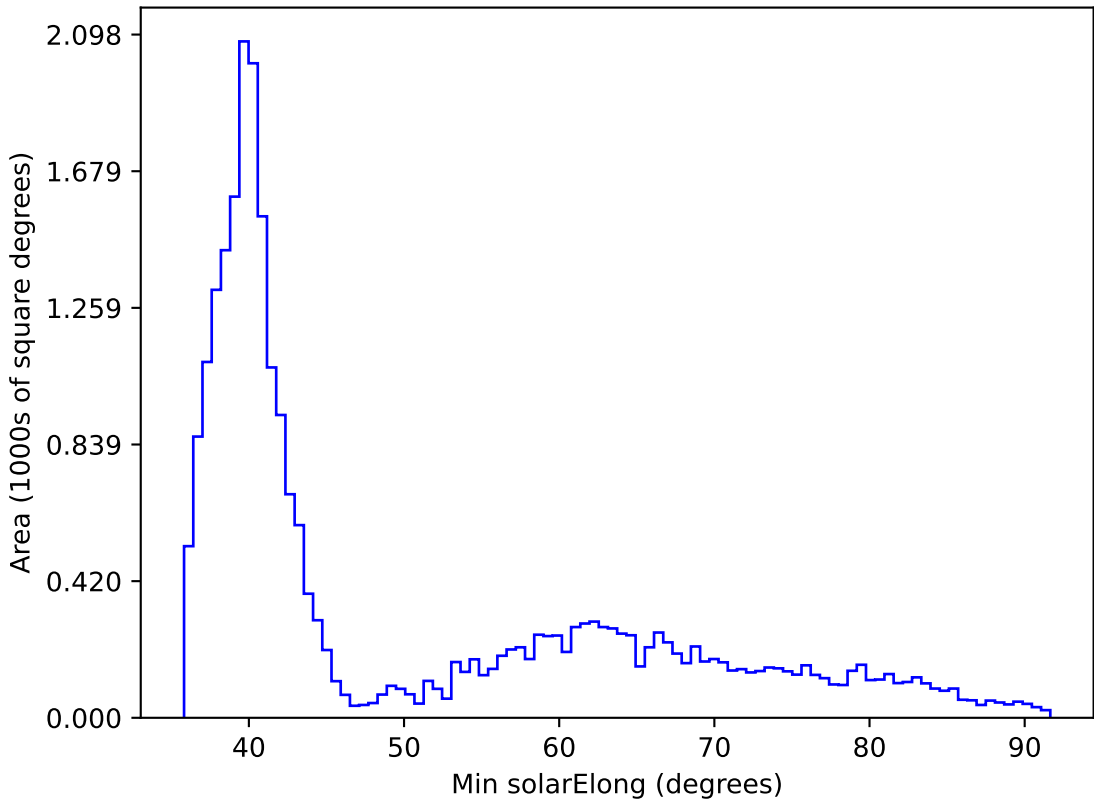
too_elab_r64_d2_gz_v3.4_10yrs All sky all bands: Min solarElong
