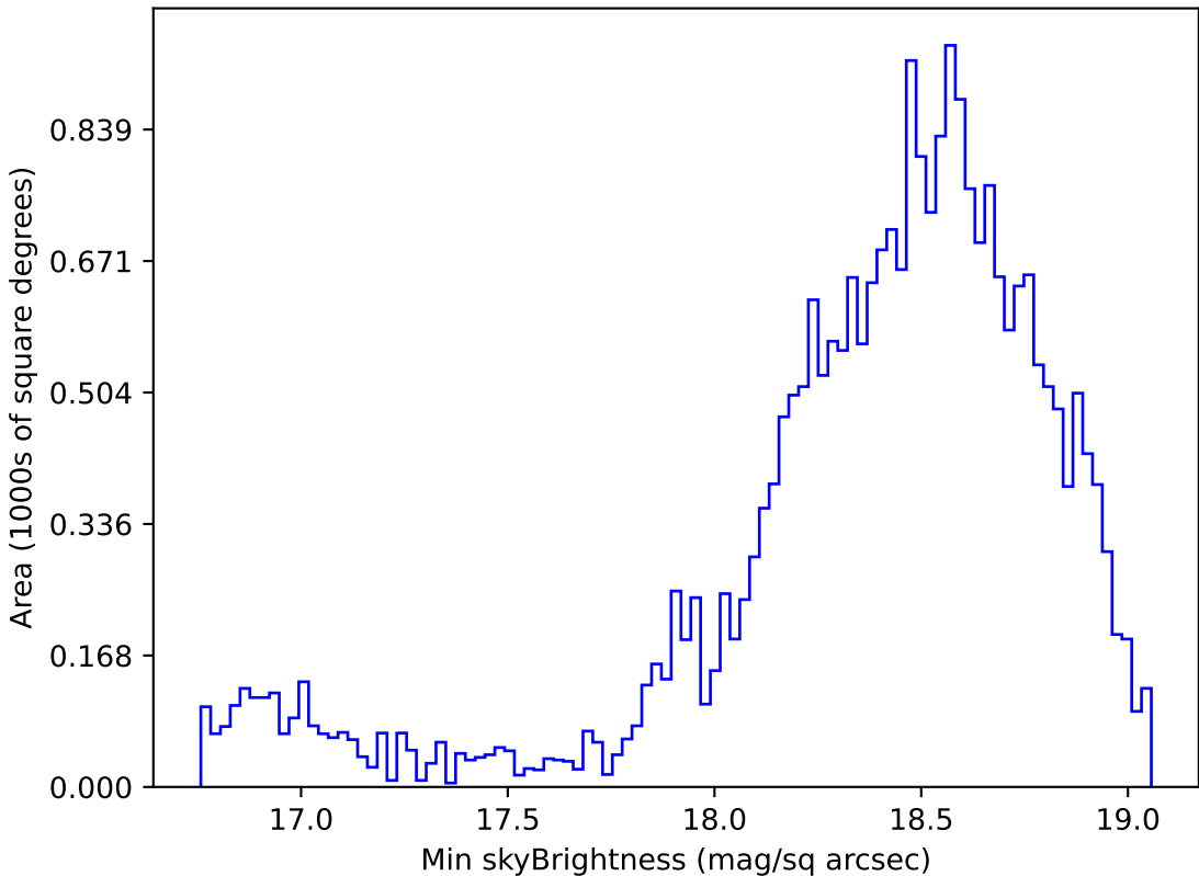
too_elab_r64_d2_gz_v3.4_10yrs Yr 1 z band: Min skyBrightness
