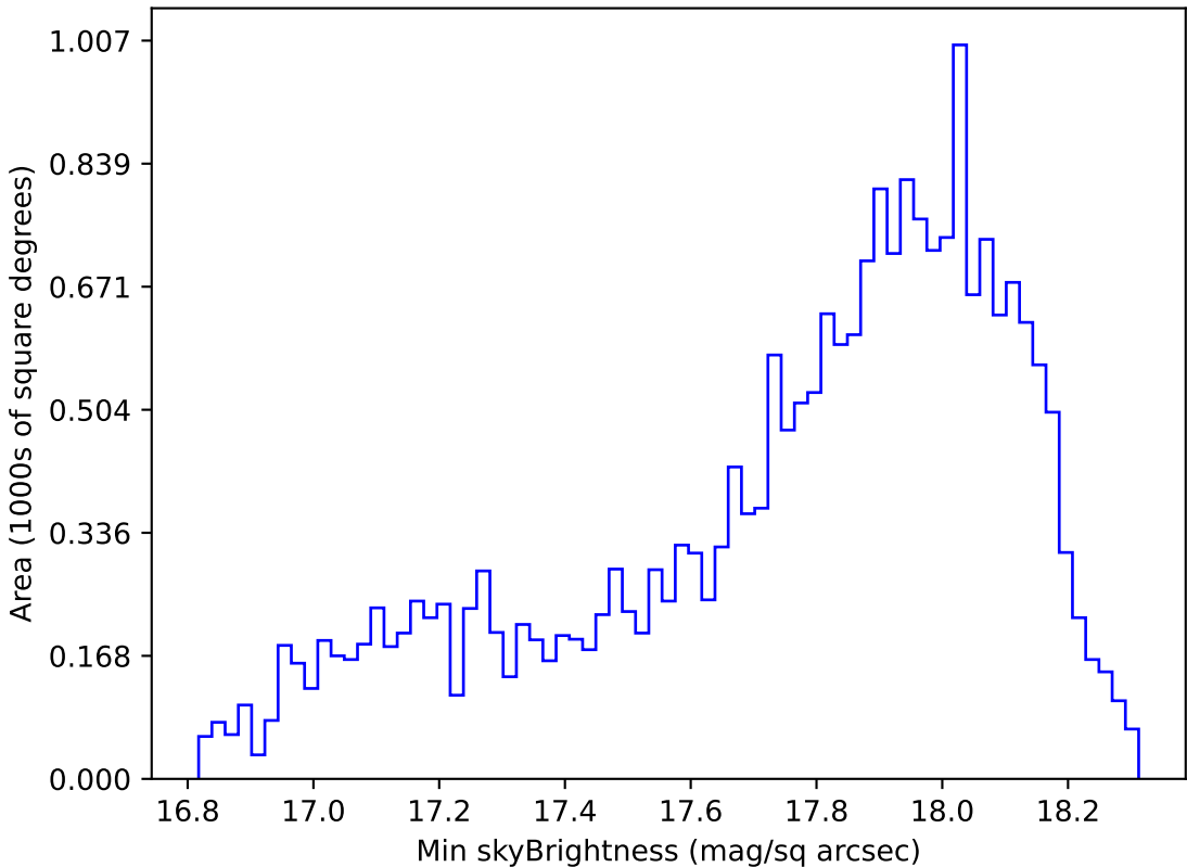
too_elab_r64_d2_gz_v3.4_10yrs Yr 1 y band: Min skyBrightness
