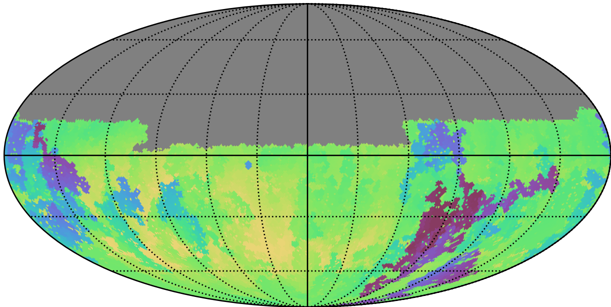
too_elab_r64_d2_gz_v3.4_10yrs Yr 1 u band: Min skyBrightness
