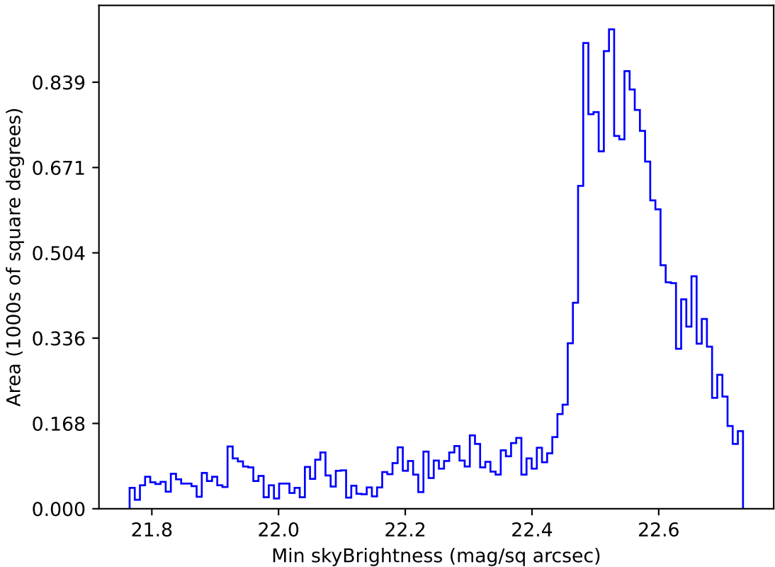
too_elab_r64_d2_gz_v3.4_10yrs Yr 1 u band: Min skyBrightness
