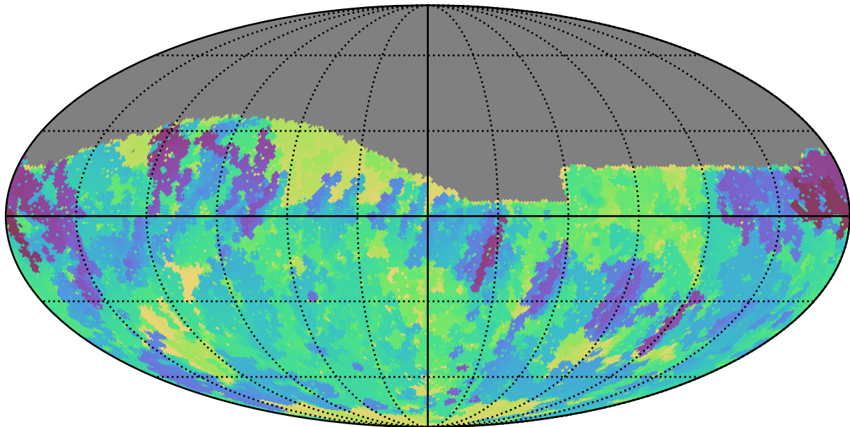
too_elab_r64_d2_gz_v3.4_10yrs Yr 1 r band: Min skyBrightness
