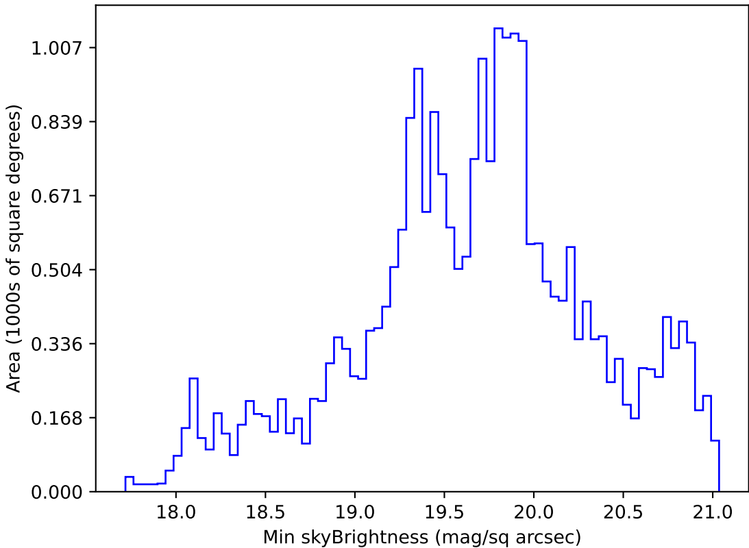
too_elab_r64_d2_gz_v3.4_10yrs Yr 1 r band: Min skyBrightness
