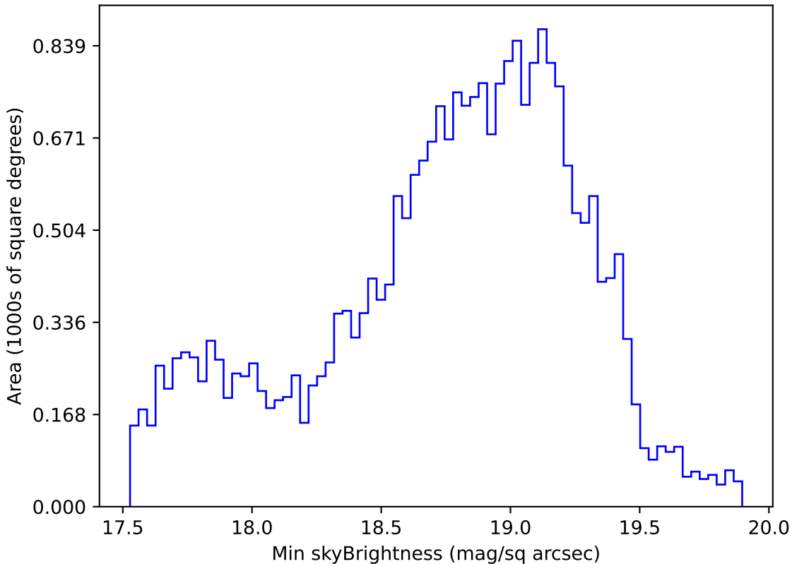
too_elab_r64_d2_gz_v3.4_10yrs Yr 1 i band: Min skyBrightness
