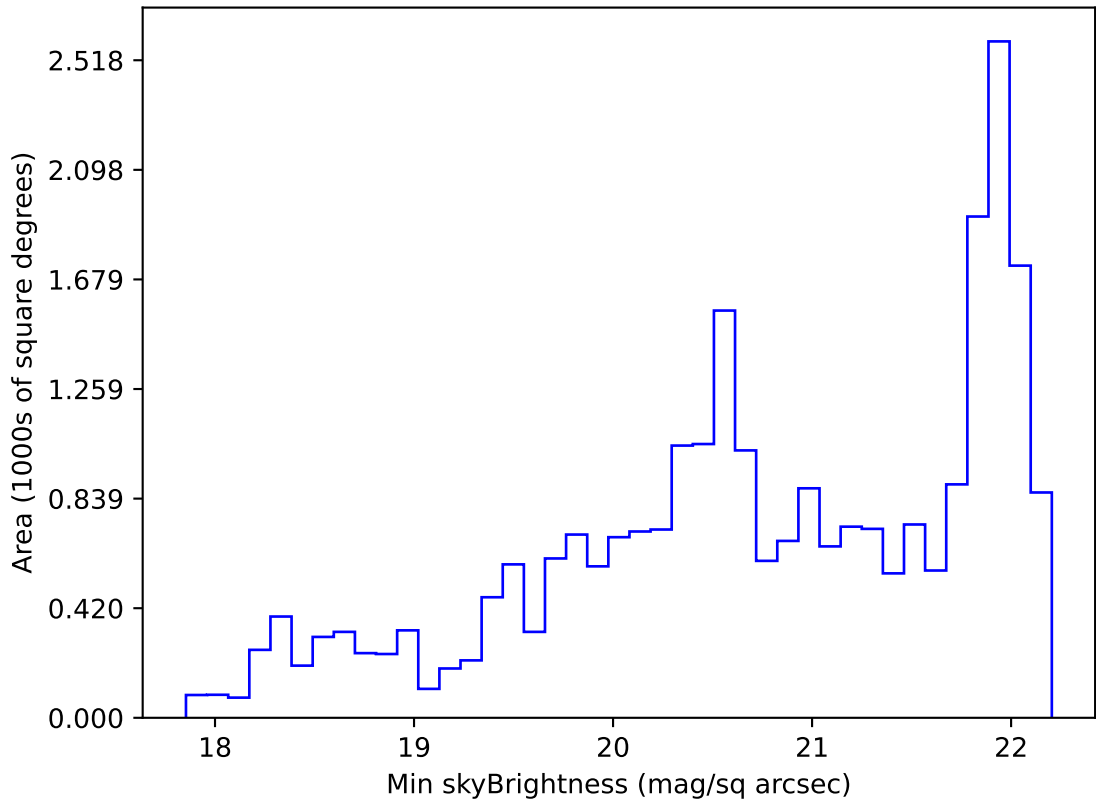
too_elab_r64_d2_gz_v3.4_10yrs Yr 1 g band: Min skyBrightness
