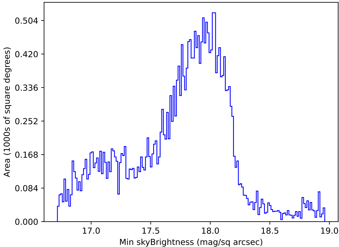
too_elab_r64_d2_gz_v3.4_10yrs Yr 1 all bands: Min skyBrightness
