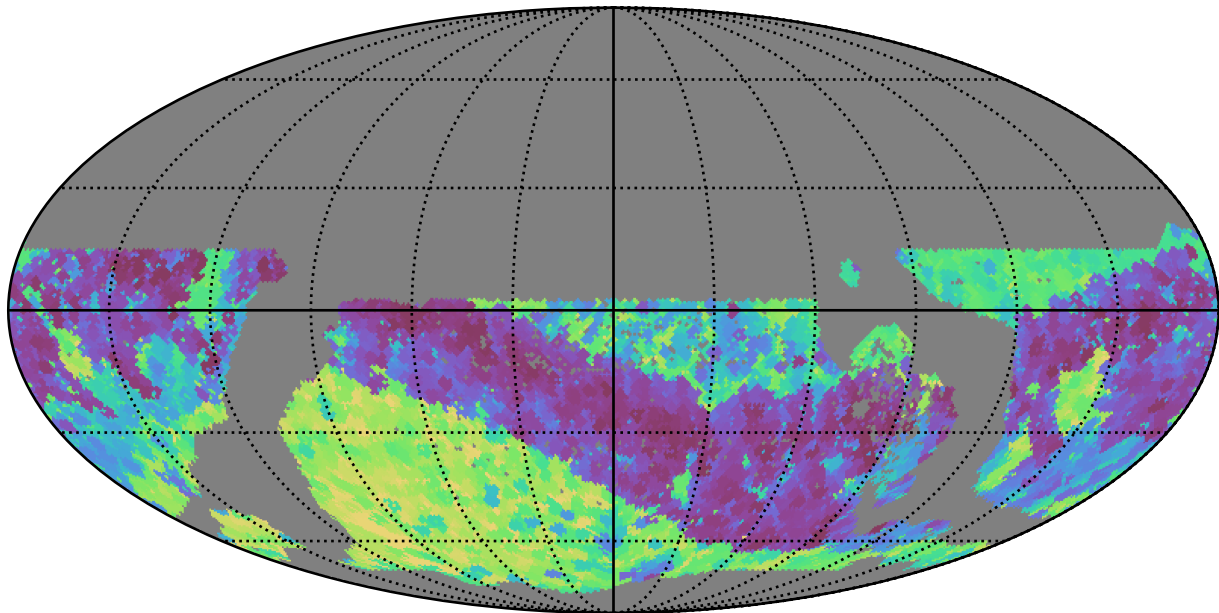
too_elab_r64_d2_gz_v3.4_10yrs WFD z band: Min skyBrightness
