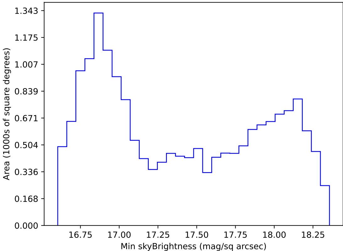
too_elab_r64_d2_gz_v3.4_10yrs WFD z band: Min skyBrightness
