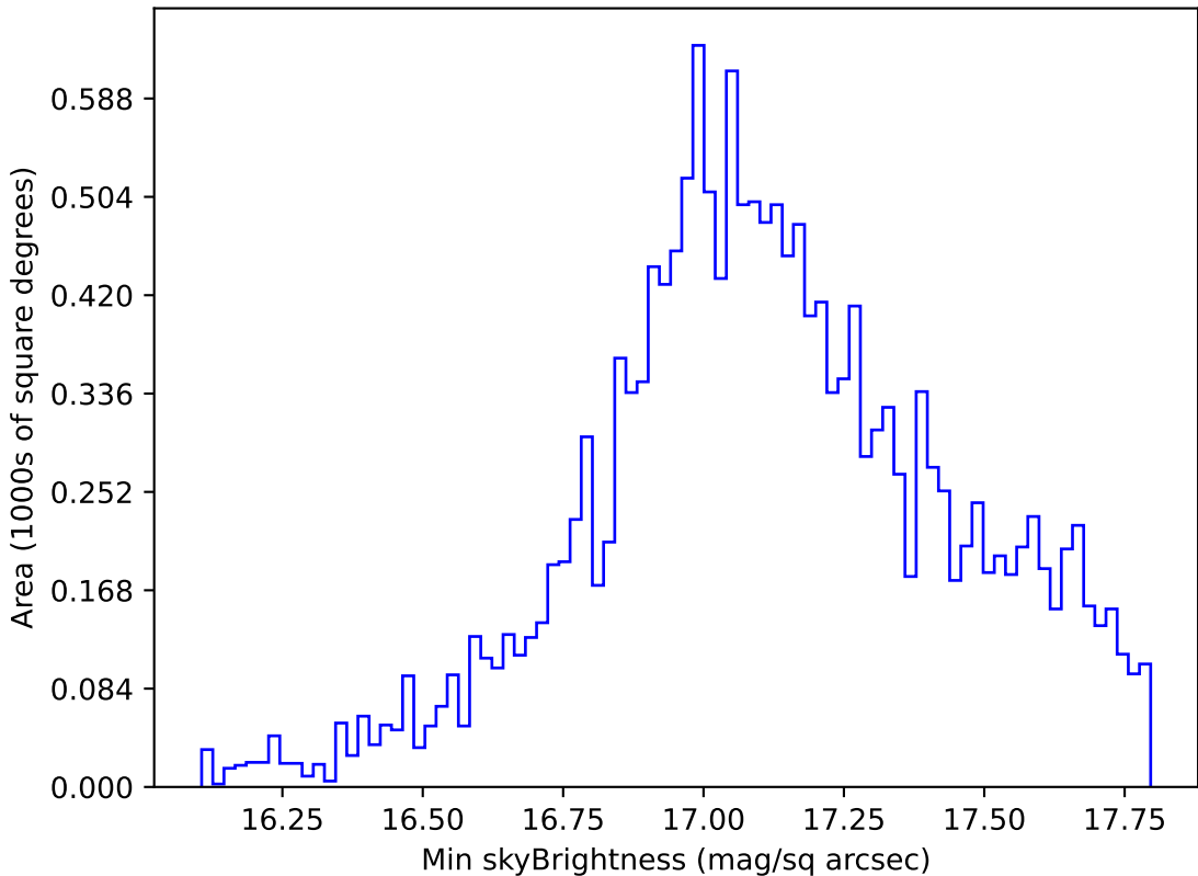
too_elab_r64_d2_gz_v3.4_10yrs WFD y band: Min skyBrightness
