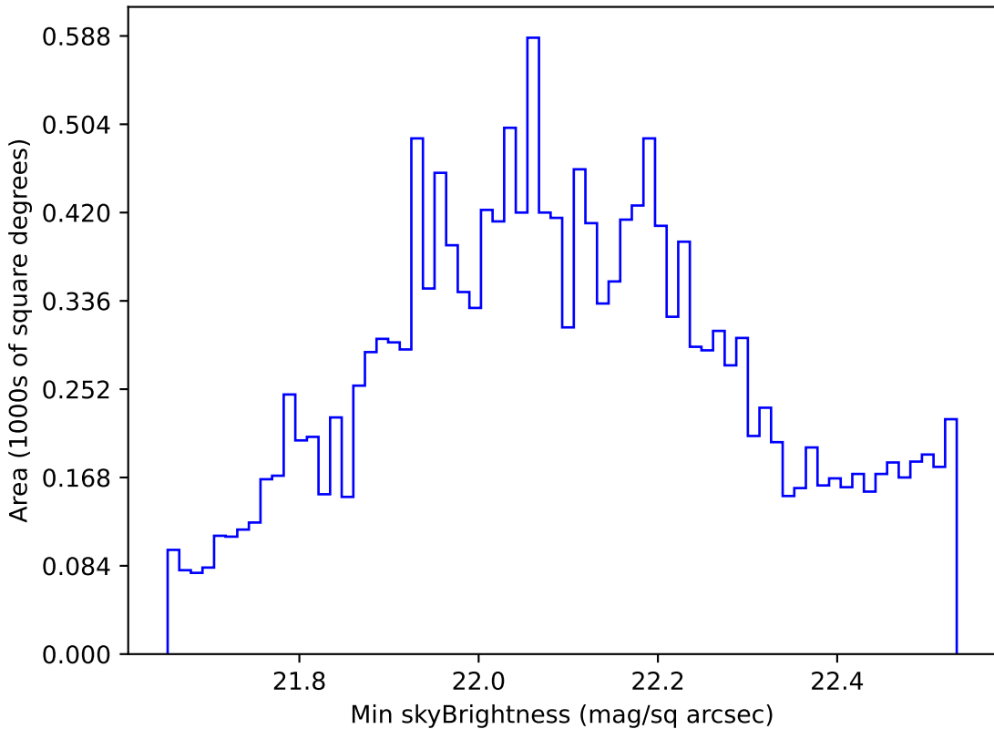
too_elab_r64_d2_gz_v3.4_10yrs WFD u band: Min skyBrightness
