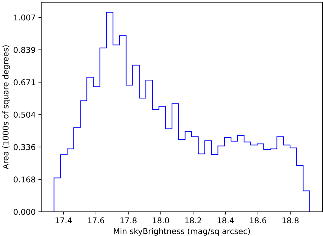
too_elab_r64_d2_gz_v3.4_10yrs WFD i band: Min skyBrightness
