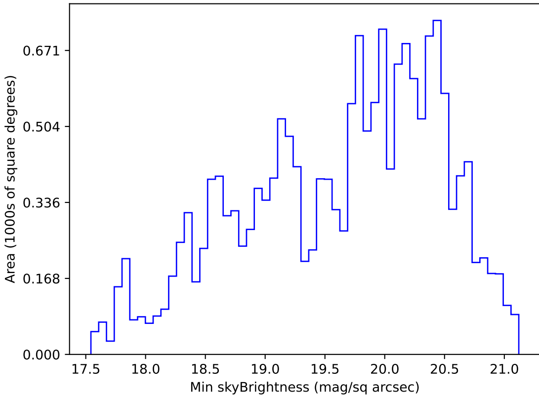
too_elab_r64_d2_gz_v3.4_10yrs WFD g band: Min skyBrightness
