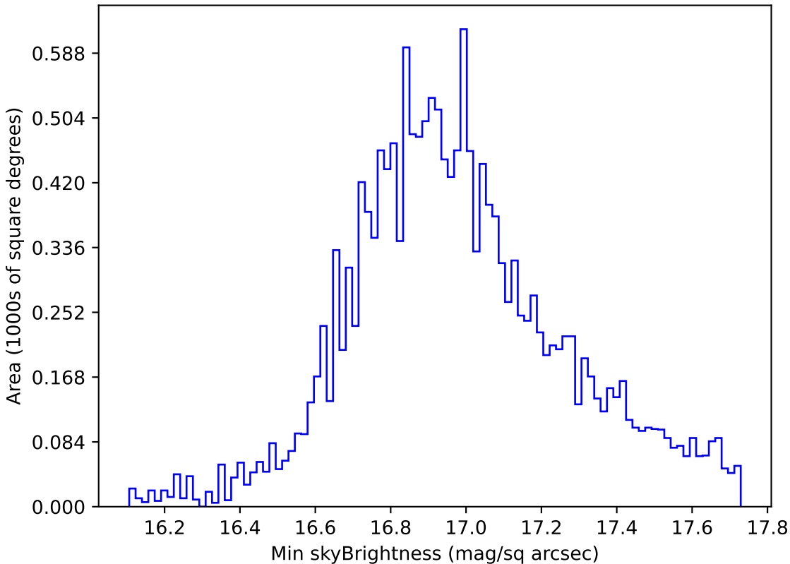
too_elab_r64_d2_gz_v3.4_10yrs WFD all bands: Min skyBrightness
