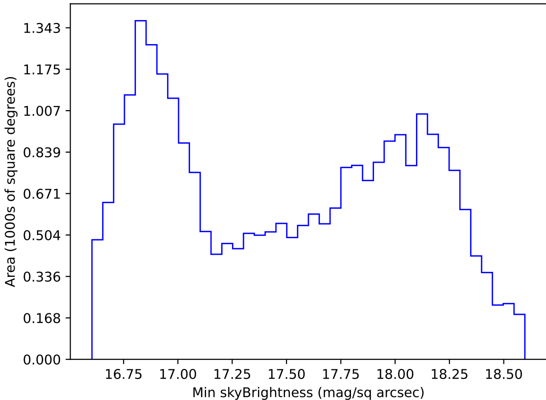
too_elab_r64_d2_gz_v3.4_10yrs All sky z band: Min skyBrightness
