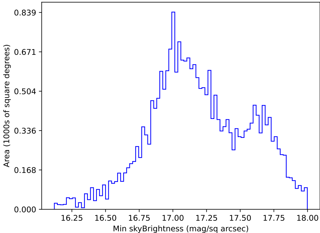
too_elab_r64_d2_gz_v3.4_10yrs All sky y band: Min skyBrightness
