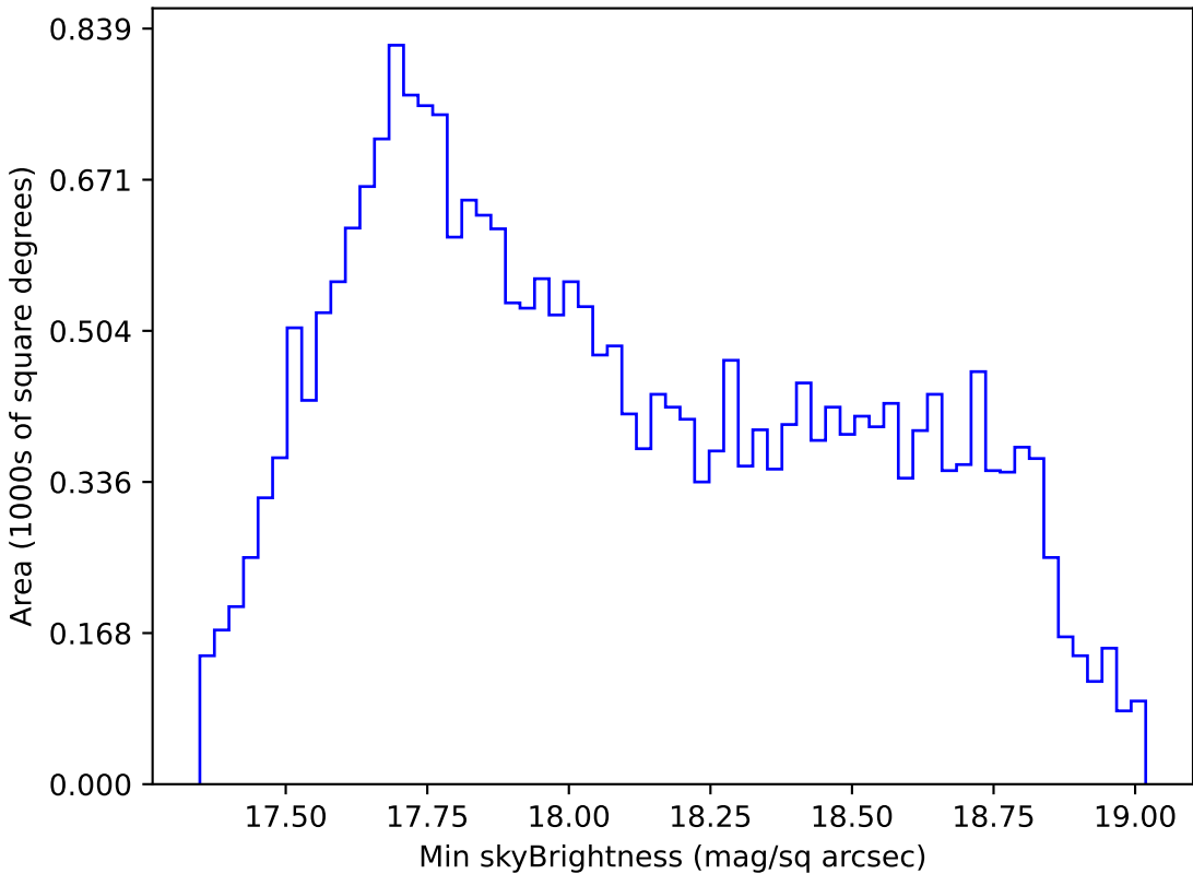
too_elab_r64_d2_gz_v3.4_10yrs All sky i band: Min skyBrightness
